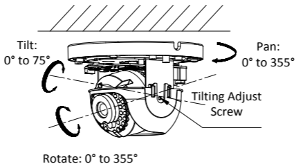
Figure 2-7 Angle Adjustment of Type II Camera
