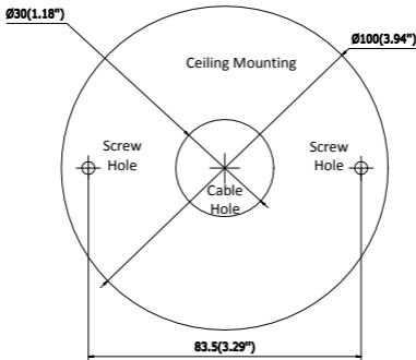
Figure 2-22 Drill Template
